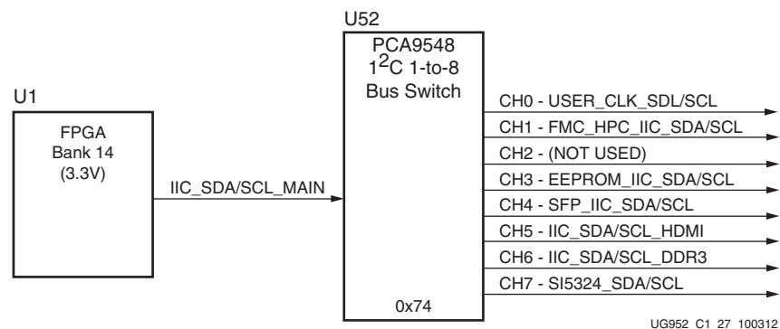
Figure 1-28: I 2 C Bus Topology
