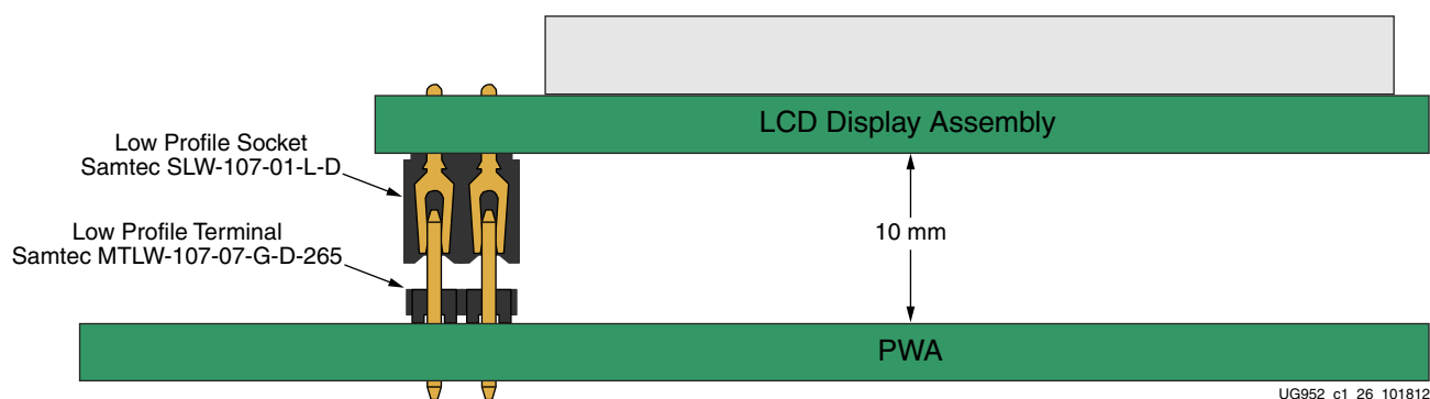
Figure 1-27: LCD Header Details
