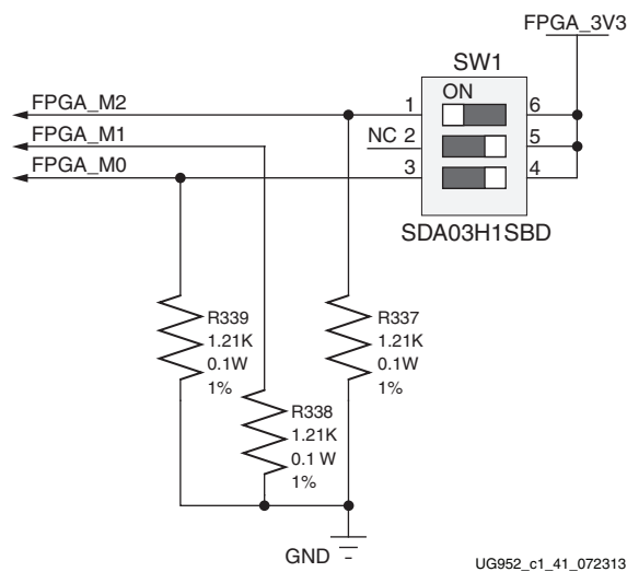
Figure 1-48: Mode Switch
