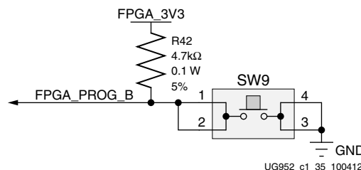
Figure 1-39: FPGA_PROG_B Pushbutton SW9
