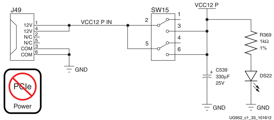
Figure 1-37: Power On/Off Switch SW15
