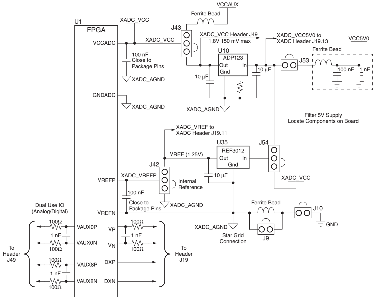
Figure 1-46: Header XADC_VREF Voltage Source Options
