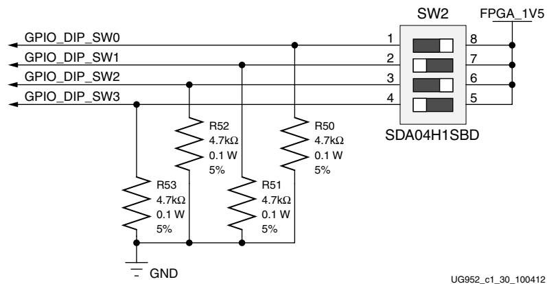
Figure 1-32: GPIO DIP Switch
