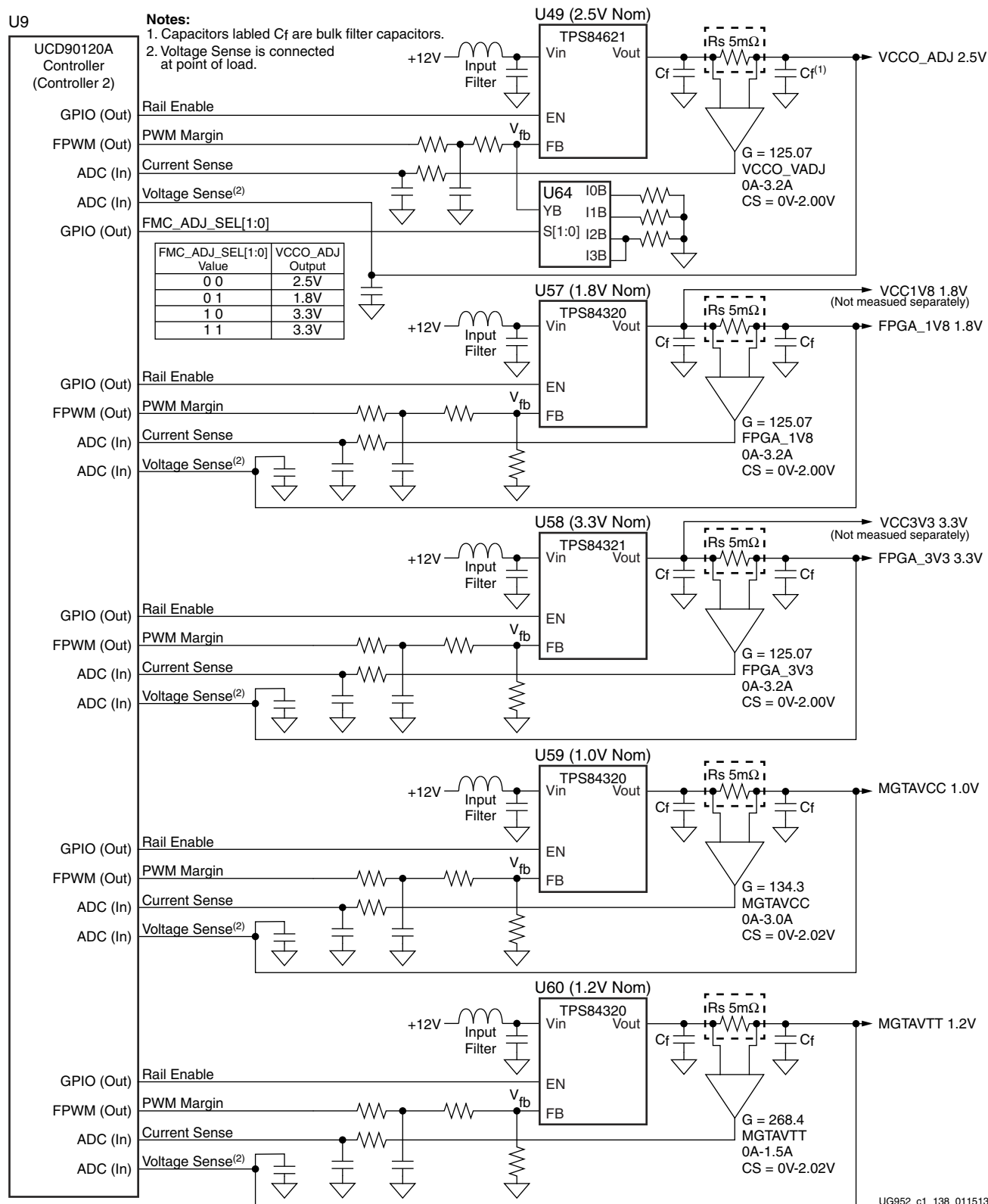
Figure 1-42: U9 Controller #2 UCD90120A Power System
