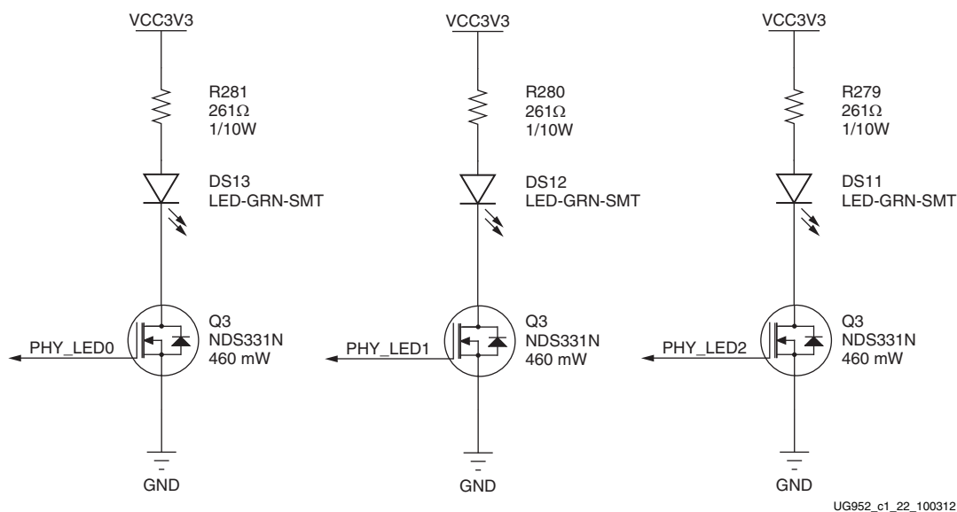
Figure 1-23: Ethernet PHY User LEDs
