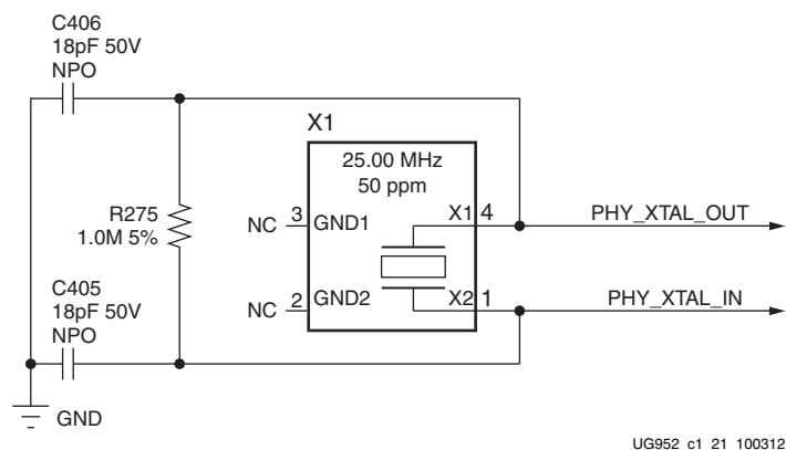
Figure 1-22: Ethernet PHY Clock Source
