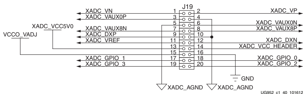
Figure 1-47: XADC header (J19)
