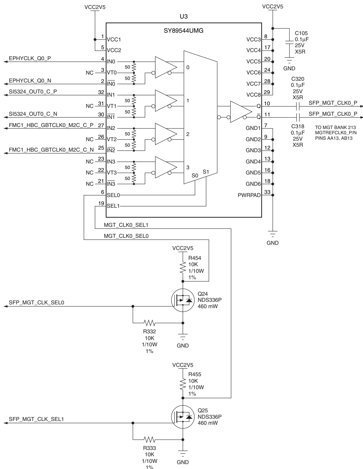
Figure 1-17: MGT Clock MUX U3 Circuit
