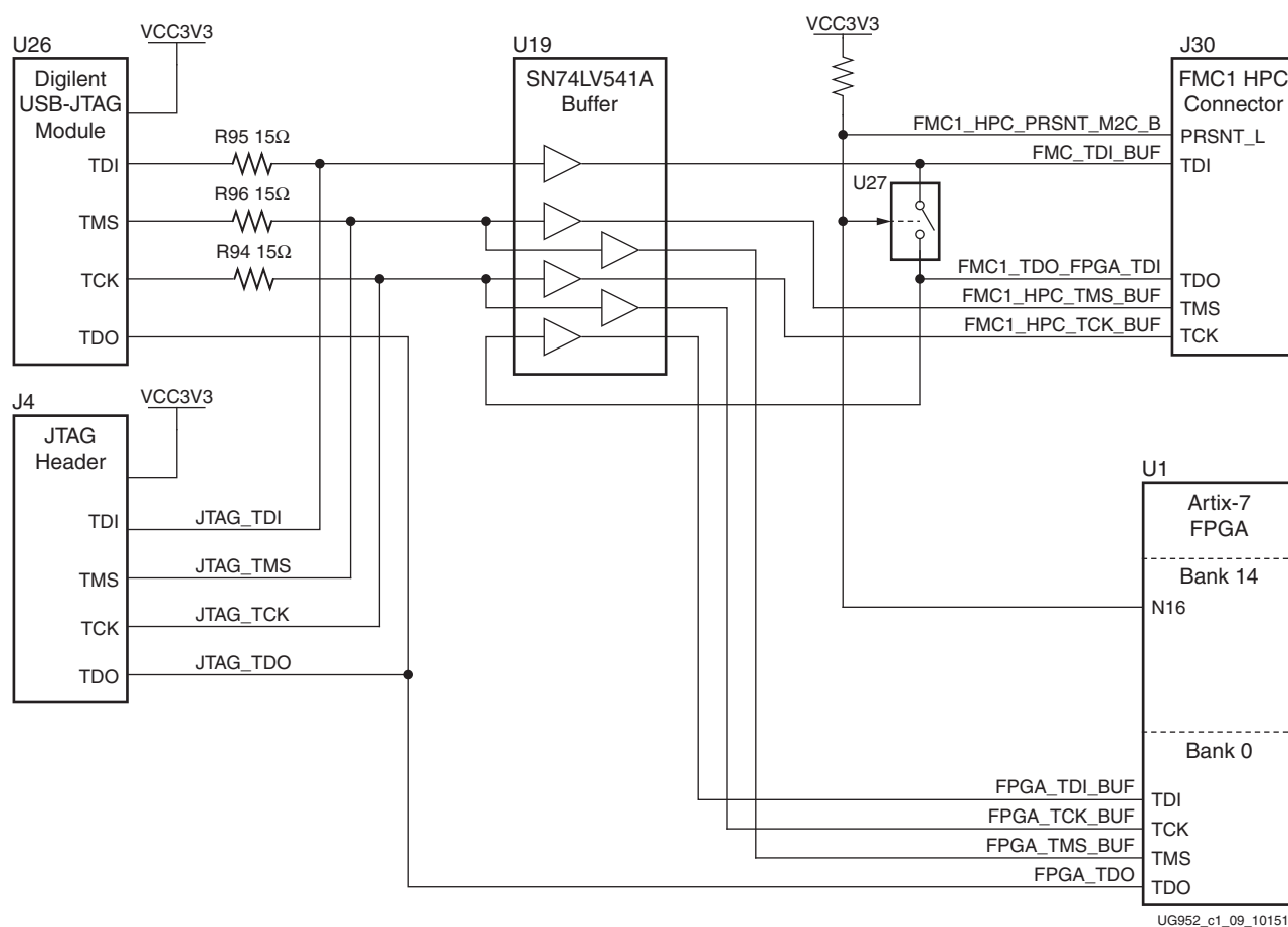
Figure 1-9: JTAG Circuit
