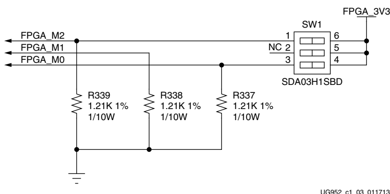
Figure 1-3: SW1 Default Settings
