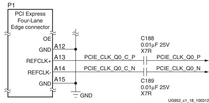
Figure 1-19: PCI Express Clock
