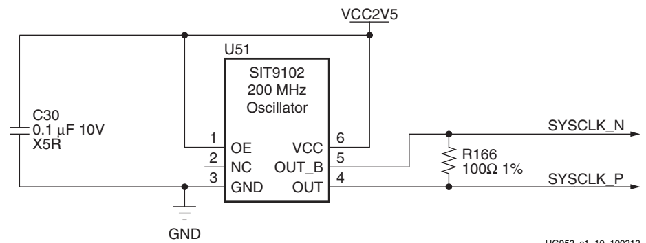
Figure 1-11: System Clock Source
