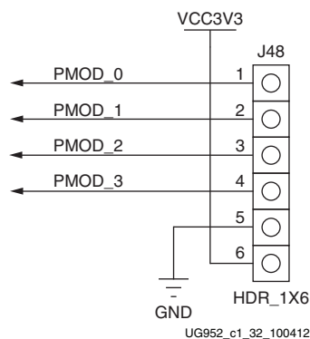
Figure 1-36: PMOD Header J48
