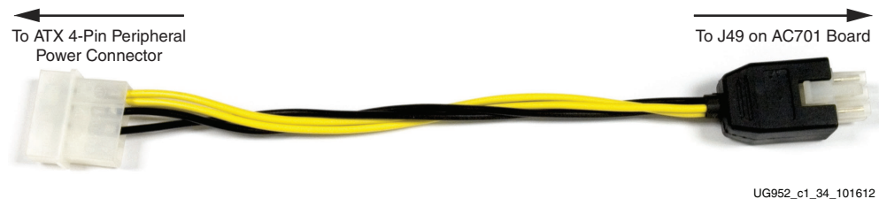
Figure 1-38: ATX Power Supply Adapter Cable
