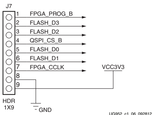
Figure 1-6: SPI J7 External Programming Connector
