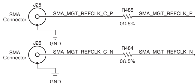
Figure 1-15: GTP SMA Clock Source
