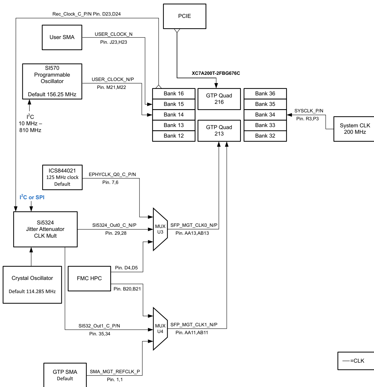
Figure 1-10: AC701 Clocking Diagram
