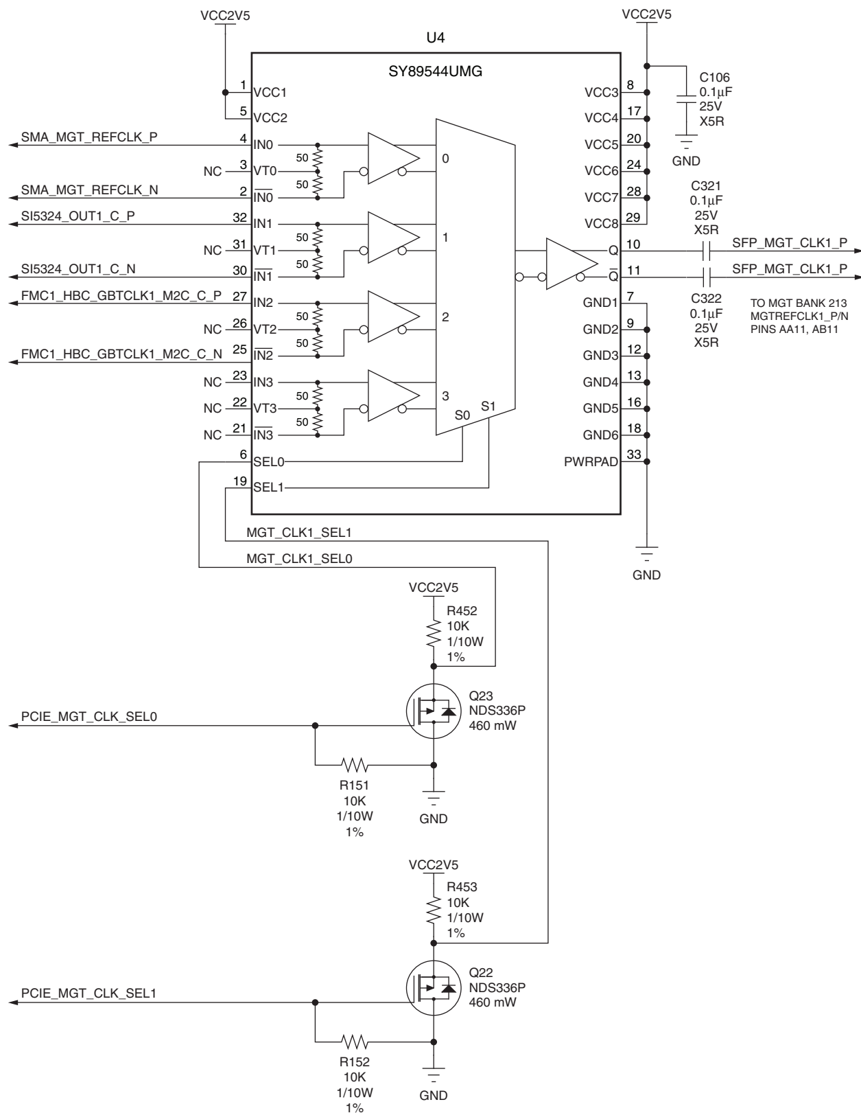
Figure 1-18: MGT Clock MUX U4 Circuit
