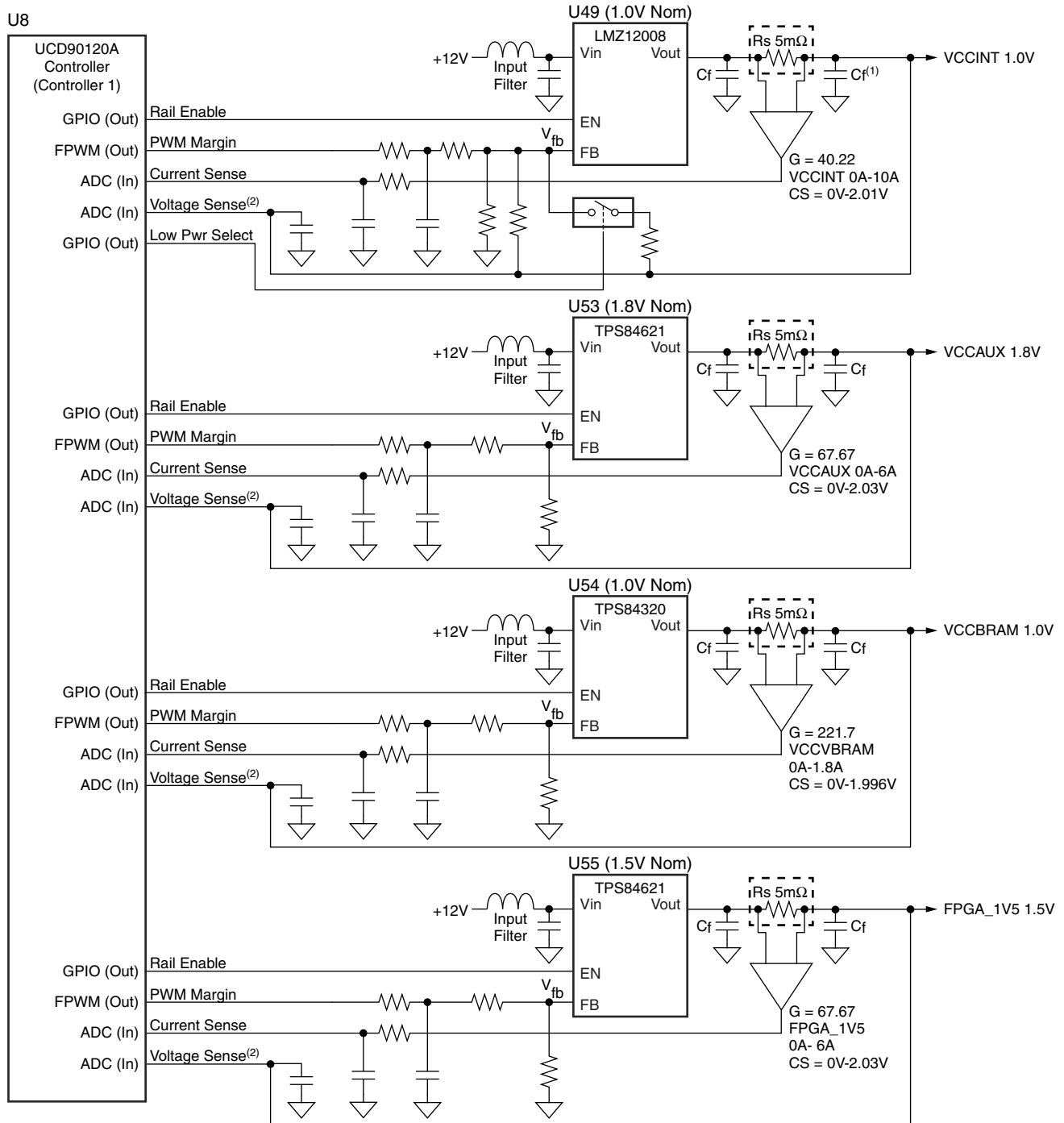
Figure 1-41 shows the power system for UCD90120A U8 controller #1
