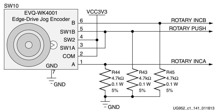
Figure 1-33: User Rotary Switch Circuit
