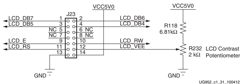
Figure 1-35: LCD Header J23
