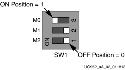
Figure A-2: SW1 Default Settings
