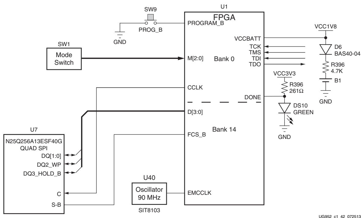
Figure 1-49: AC701 Board QSPI Configuration Circuit
