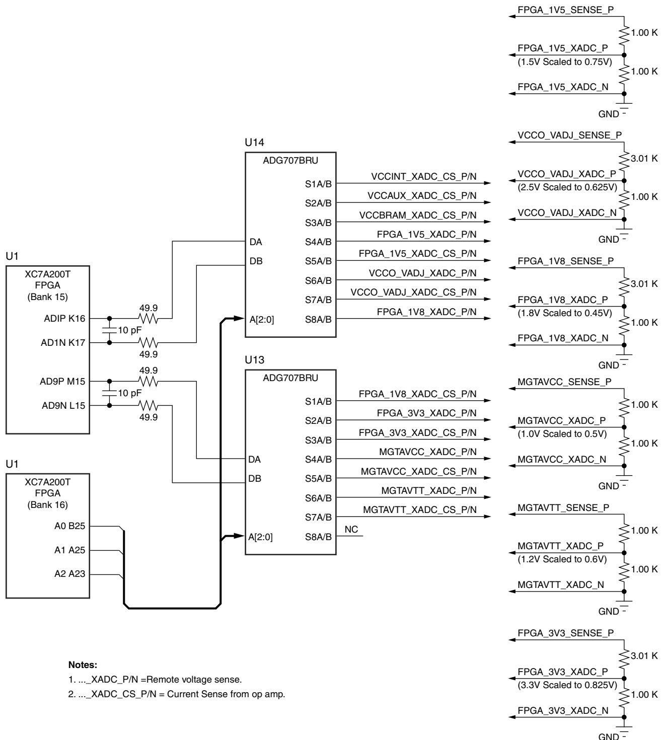
Figure 1-43: XADC External Multiplexer Block Diagram
