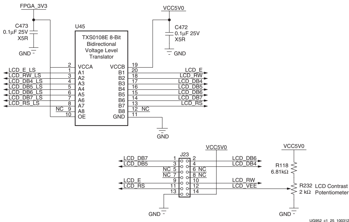
Figure 1-26: LCD Interface Circuit
