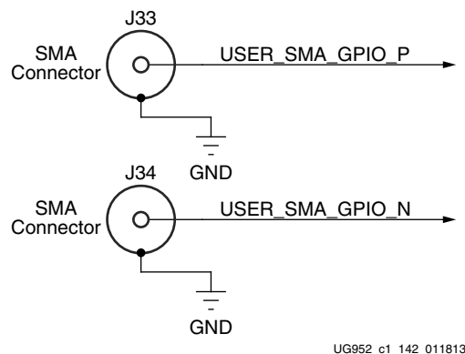
Figure 1-34: User SMA Connector
