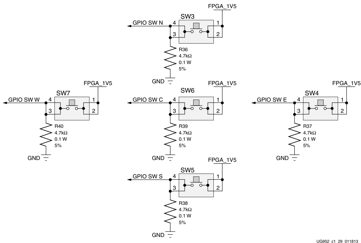
Figure 1-30: User Pushbuttons
