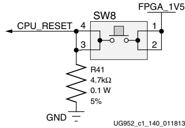
Figure 1-31: CPU_RESET Pushbutton
