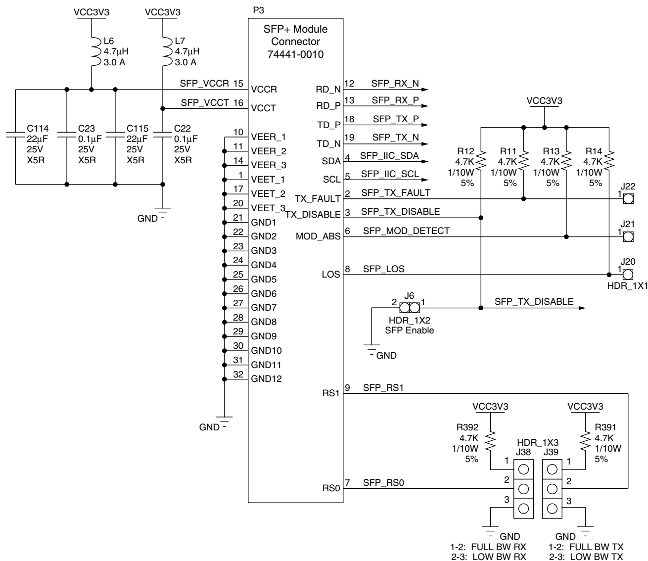
Figure 1-21: SFP+ Module Connector
