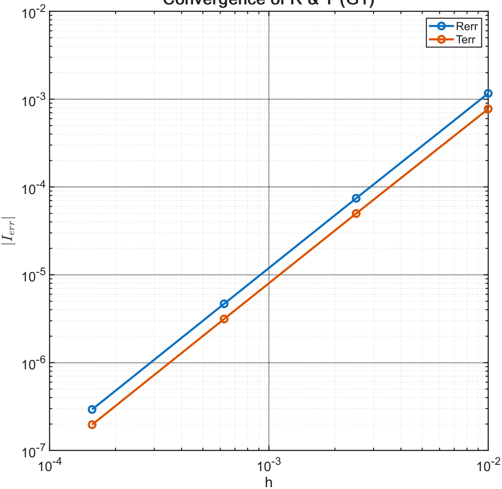
Convergence of R & T (G1)
