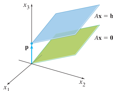
FIGURE 6 Parallel solution sets of A\mathbf{x} = \mathbf{b} and A\mathbf{x} = \mathbf{0} .
