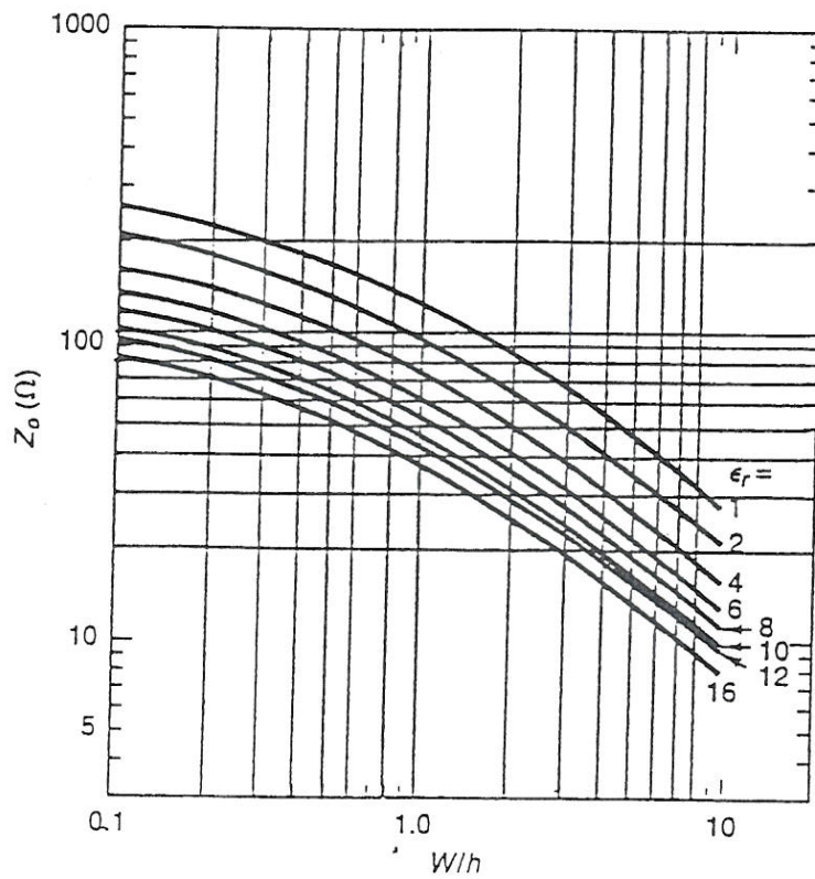
Characteristic impedance of the microstrip line versus W/h .
