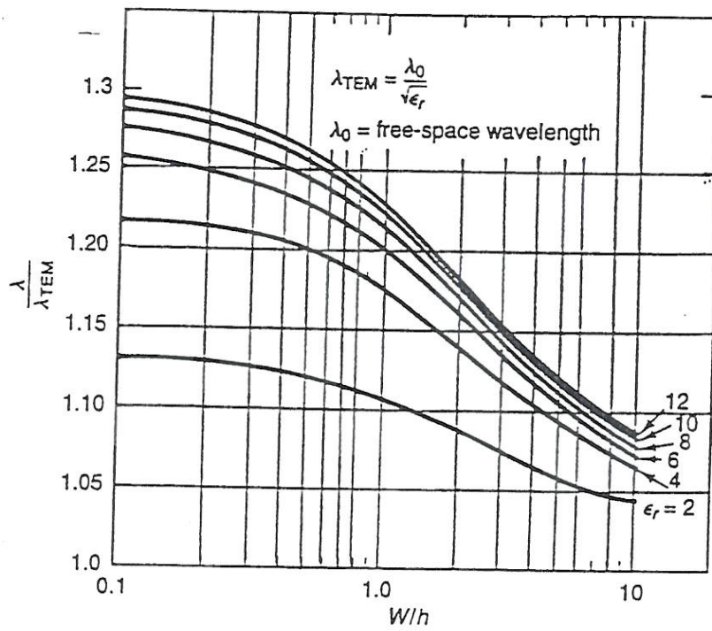
Normalized wavelength of the microstrip line versus W/h .
